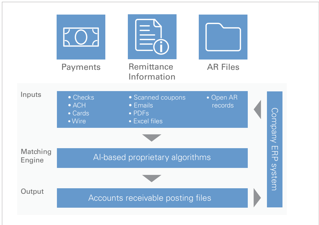
DadePay AR Automation workflow
